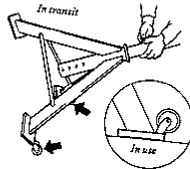
Figure 38 - Wheels avoid carrying when moving
