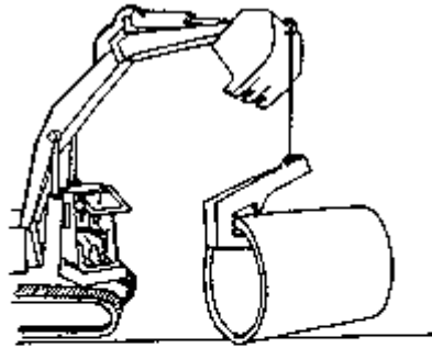
Figure 52 - Using c-hook to move cylinders and pipes
