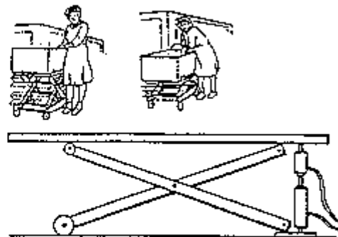
Figure 50 - Adjustable scissor table for different work heights
