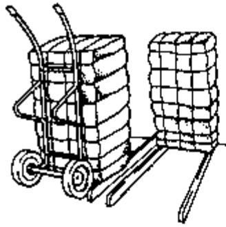
Figure 35 - Rails enable trolleys to slide under loads
