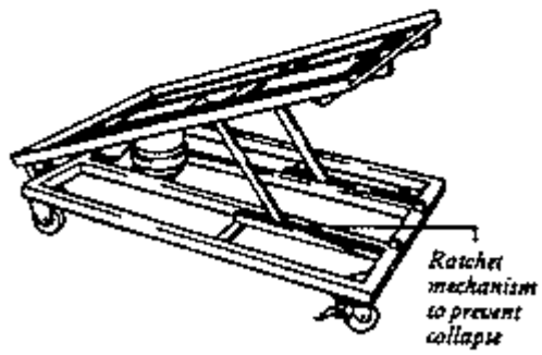
Figure 45 - Rolling platform with tilt mechanism
